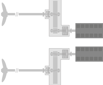
RENK standard mechanical propulsion solution
