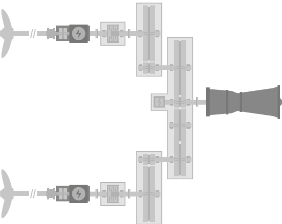
RENK hybrid propulsion solution
